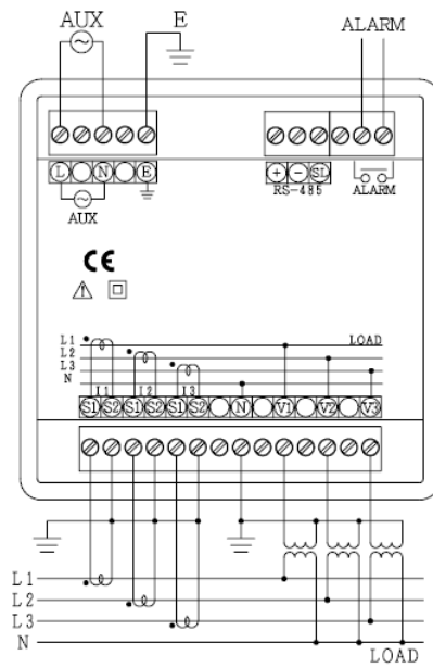
(a) XS-96-M
