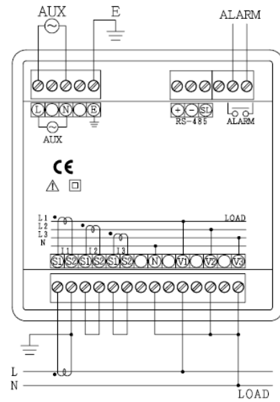
(a) XS-96-M
