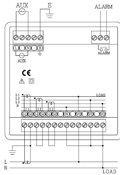
(b) XS-96-0
