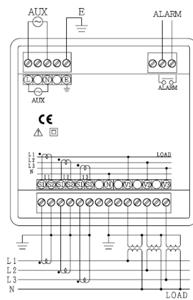
(b) XS-96-0
